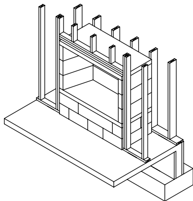
Vent-Free Series with raised hearth
