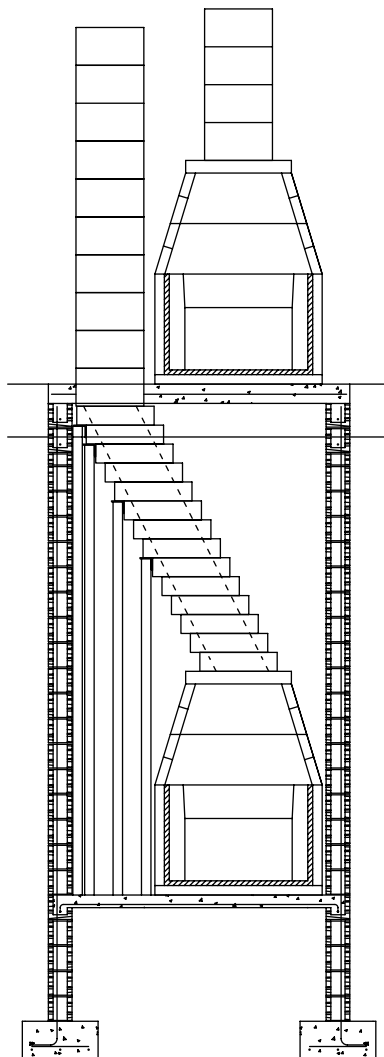
Stacked fireplace application
