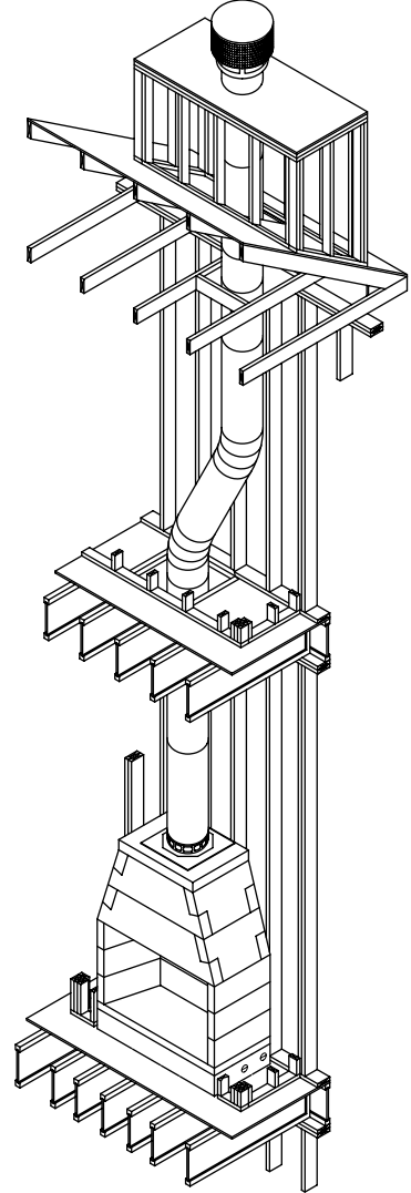
Fire-Lite Series with Metal Chimney
