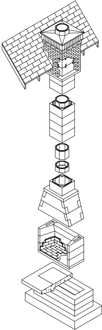
Standard Series with DM Chimney
